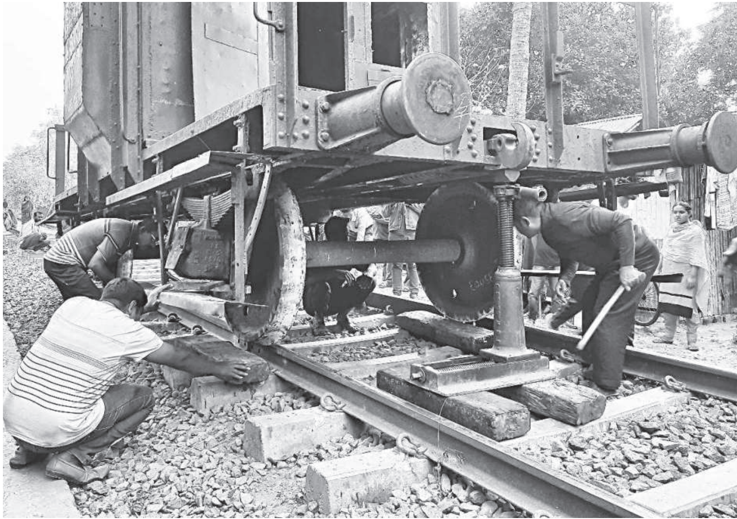
Workers were busy removing the compartment of an oil-laden train that got derailed in Khulna yesterday afternoon. The accident took place around 2:10pm in front of BGB headquarters in Daulatpur area. Rail connection was re-established around 8:00pm. PHOTO: HABIBUR RAHMAN
