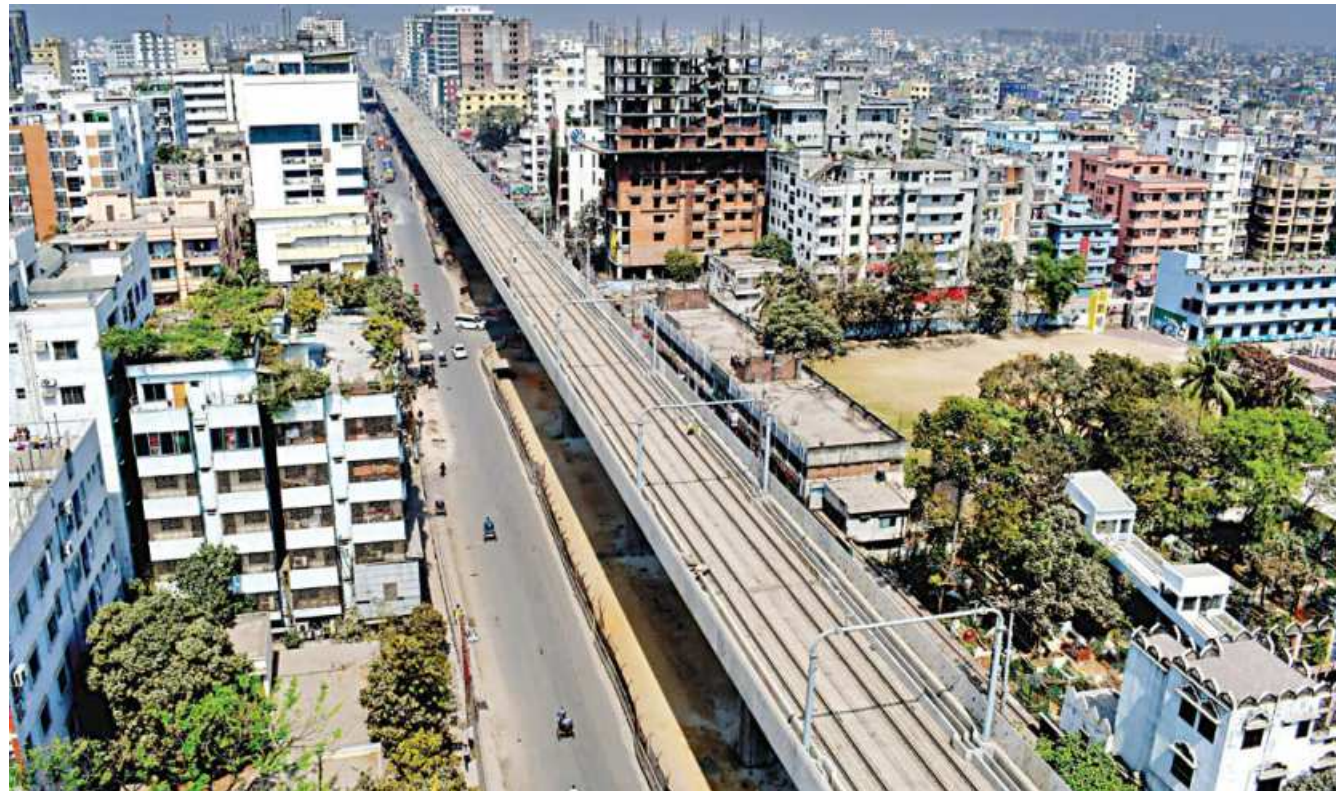
The first phase of the metro rail project -- Uttara to Agargaon -- is now visible in its entirety as the last viaduct of this part was installed yesterday. The photo was taken near Mirpur 11 yesterday.
