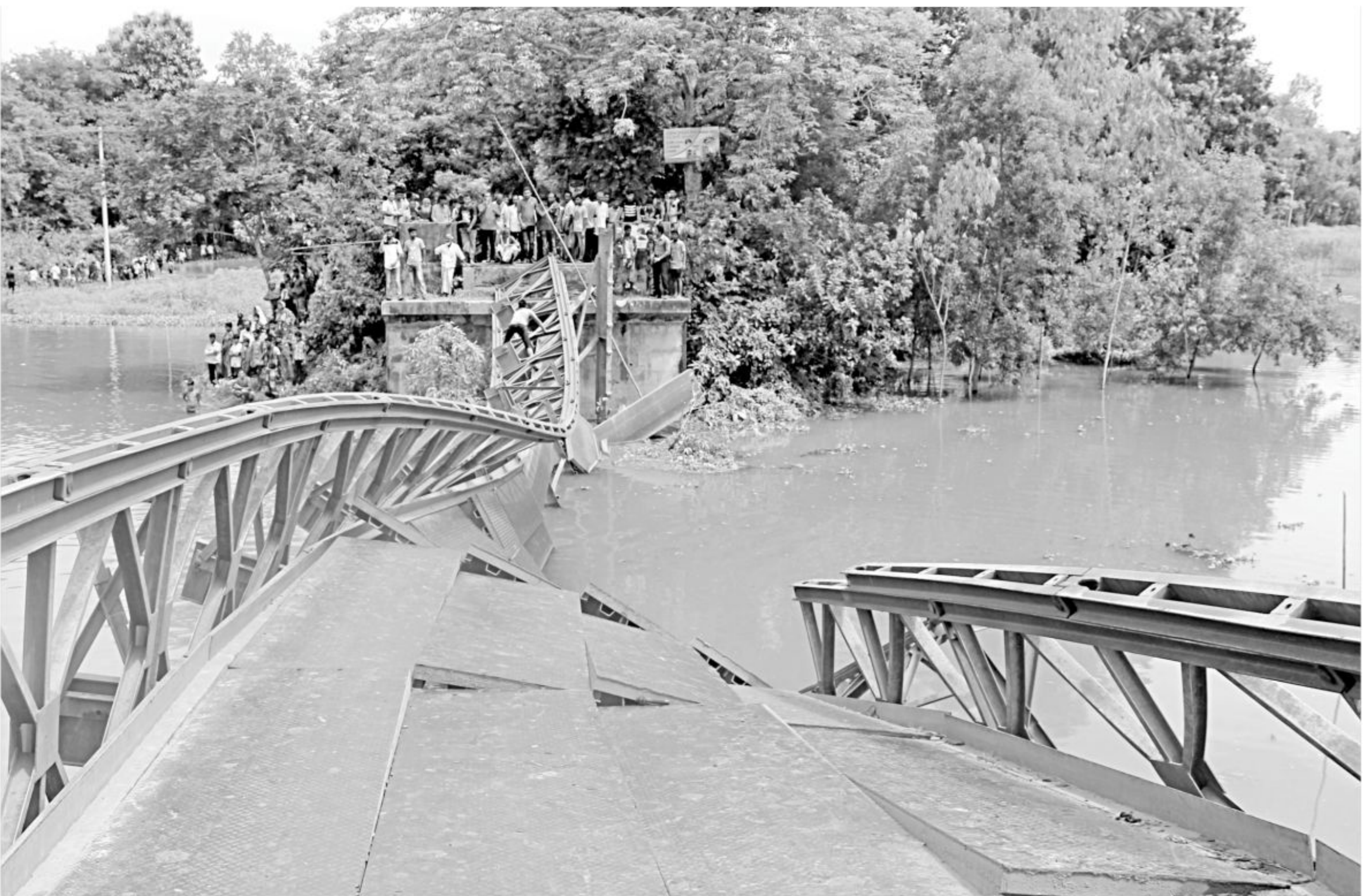
A Bailey bridge on a canal in Dulla area of Tangail's Delduar upazila collapses under pressure of a fertiliser-laden truck yesterday. PHOTO: MIRZA SHAKIL
