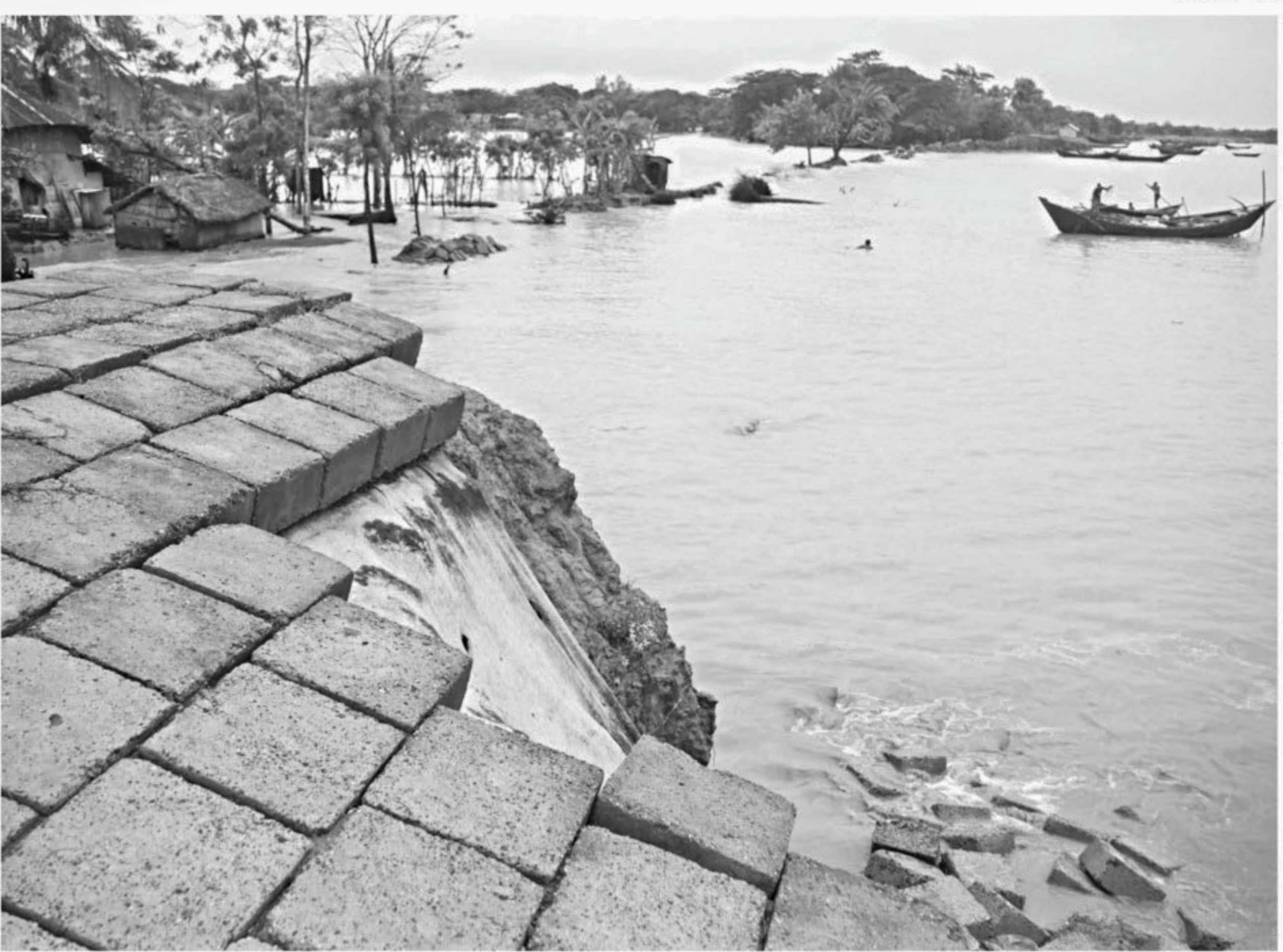
This embankment on the Andharmanik River at Nizampur village in Kuakata area of Patuakhali district collapsed under the pressure of tidal water during the new moon a couple of days ago, inundating five villages in the nearby area. The tidal surges flooded over a hundred villages and around 50 coastal islands in the district, much to the sufferings of tens of thousands of people.
