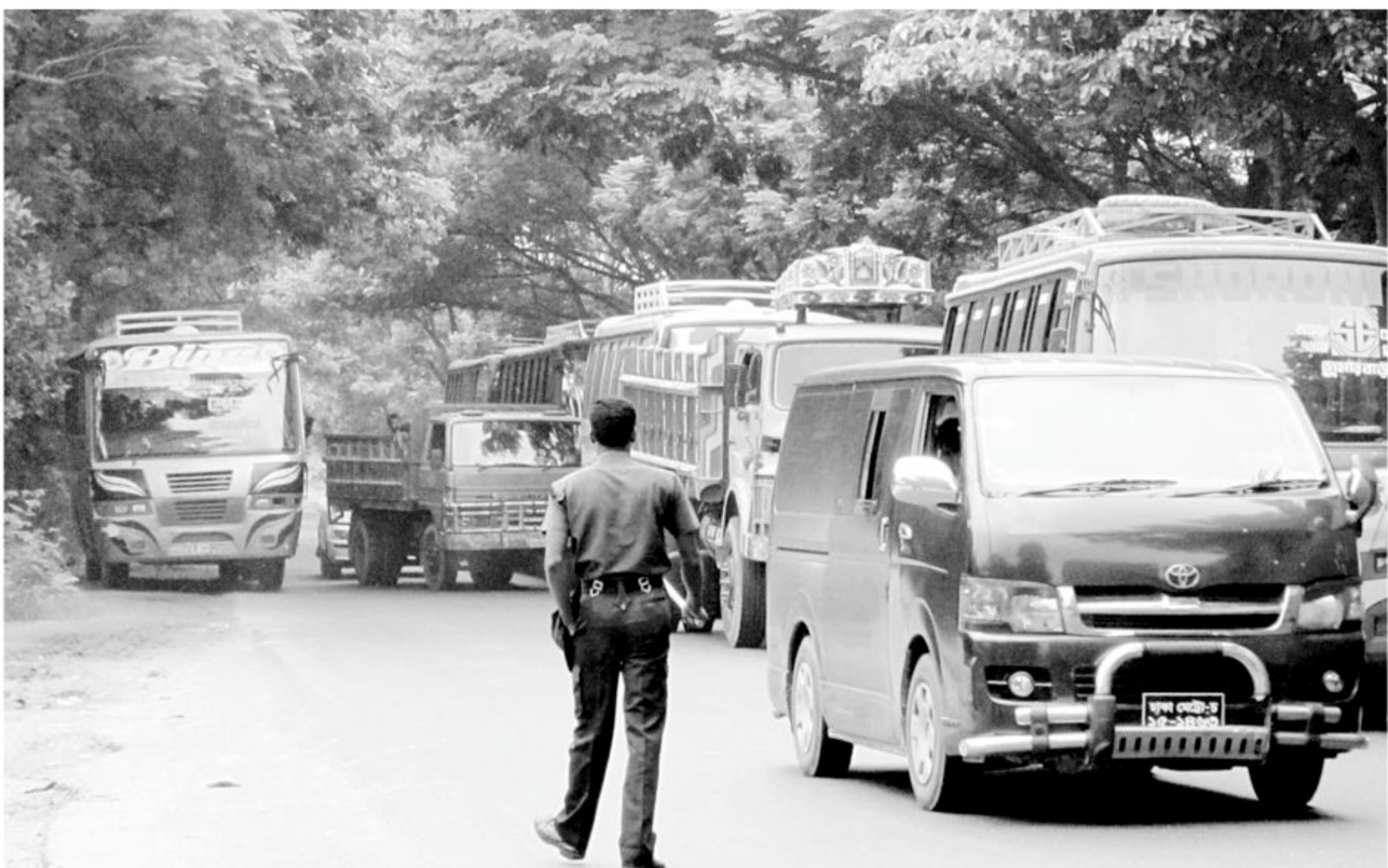
PHOTO: STAR
