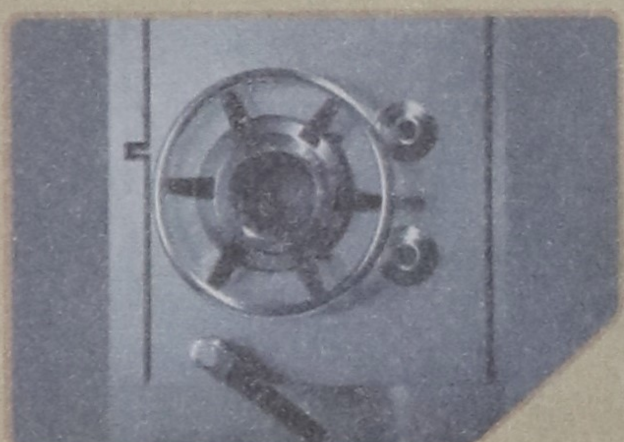
4-Stage Security
