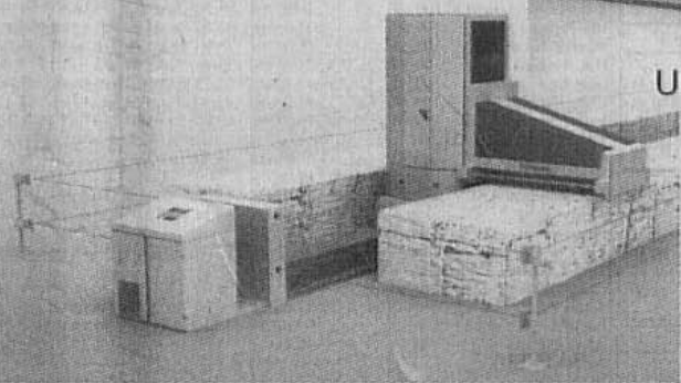
AUTOMATIC BALE OPENER BO-A
