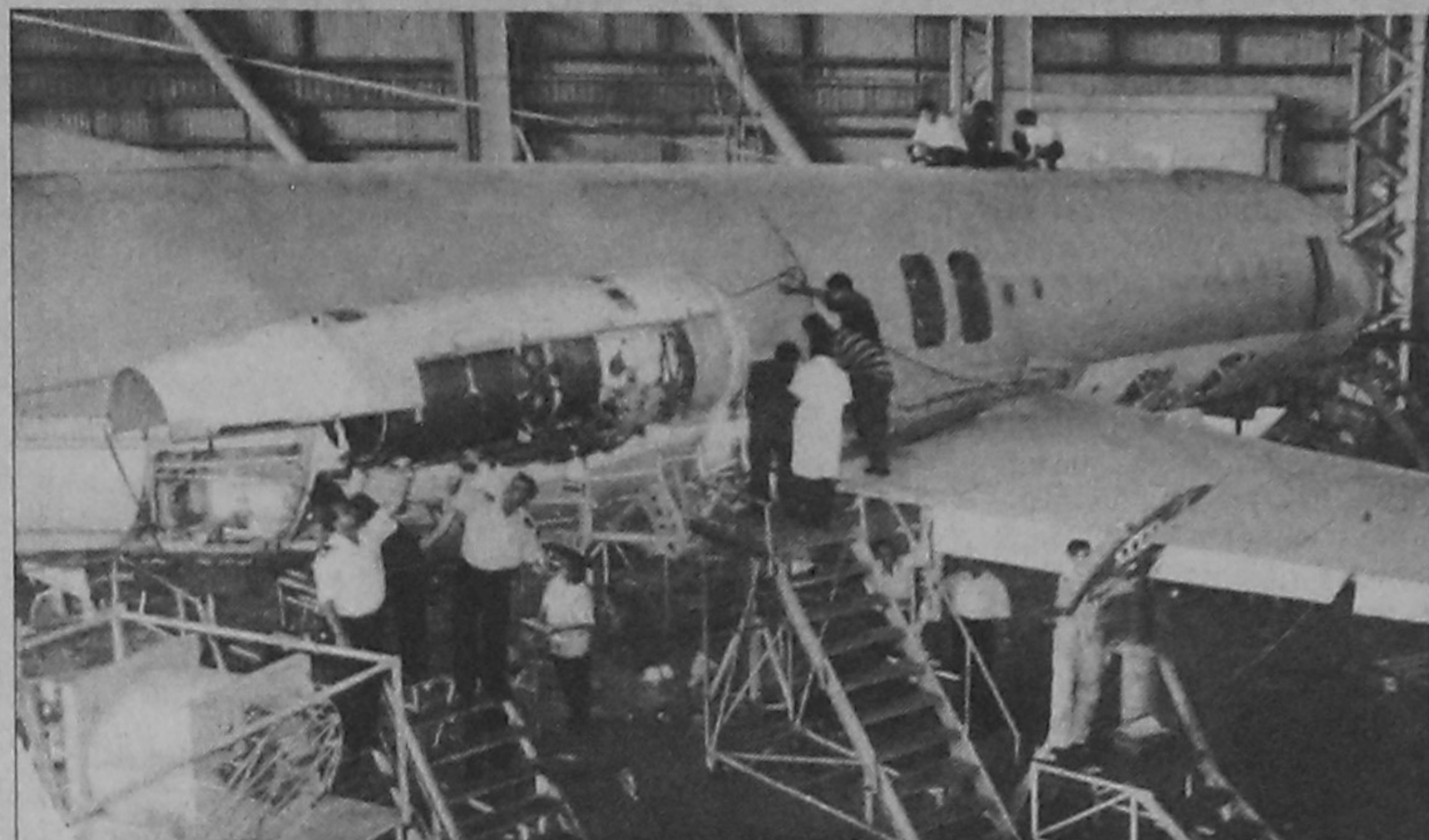
Photo shows Biman's engineers and technicians performing D-check on an F-28 aircraft in the Biman Engineering Hanger Complex at Kurmitola in the city. This is the second time Biman's engineers and technicians are carrying out D-checks on its F-28 aircraft which will save a huge amount in foreign exchange.
