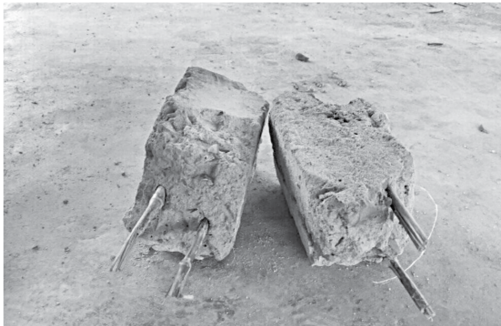
Bamboos instead of iron rods have been used in construction of the toilet of Baithakata Government Primary School in Barguna's Amtali upazila. It collapsed on Saturday.
